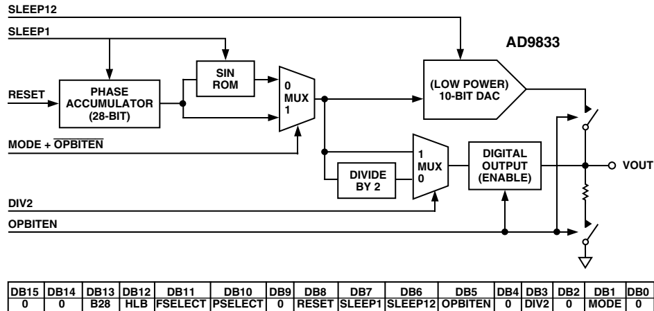
Figure 5. Function of Control Bits
