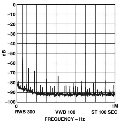
TPC 13. f_{MCLK} = 25 \text{ MHz} , f_{OUT} = 60 \text{ kHz} , Frequency Word = 009D495
