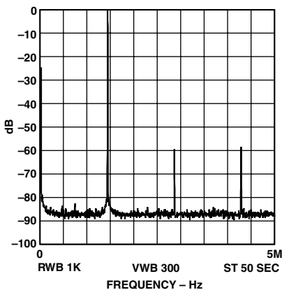
TPC 10. f_{MCLK} = 10 \text{ MHz} , f_{OUT} = 1.43 \text{ MHz} = f_{MCLK}/7 , Frequency Word = 2492492
