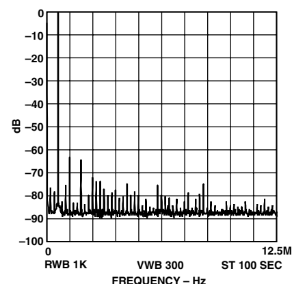
TPC 14. f_{MCLK} = 25 \text{ MHz} , f_{OUT} = 600 \text{ kHz} , Frequency Word = 0624DD3
