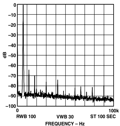
TPC 9. f_{MCLK} = 10 \text{ MHz} , f_{OUT} = 2.4 \text{ kHz} , Frequency Word = 000FBA9
